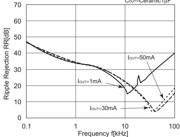
R1180x361x
