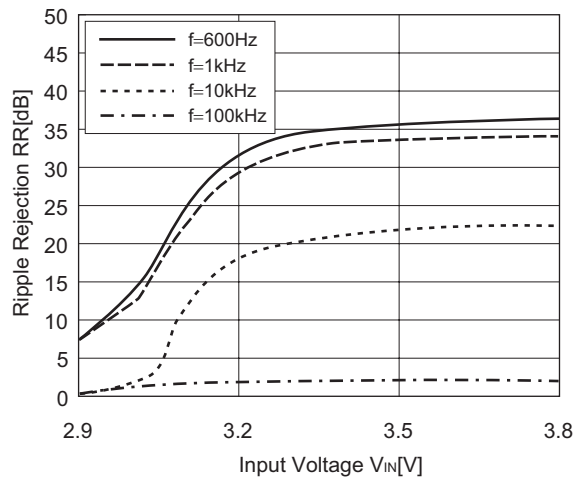
R1180x281x( I_{OUT}=30\text{mA} )
