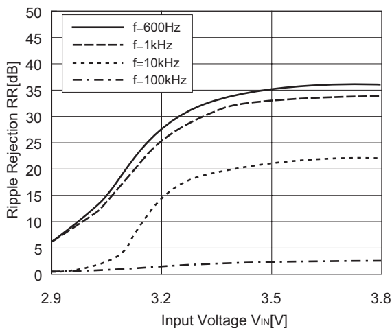
R1180x281x( I_{OUT}=50\text{mA} )
