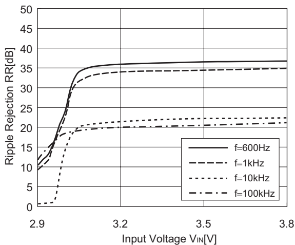
R1180x281x( I_{OUT}=50\text{mA} )
